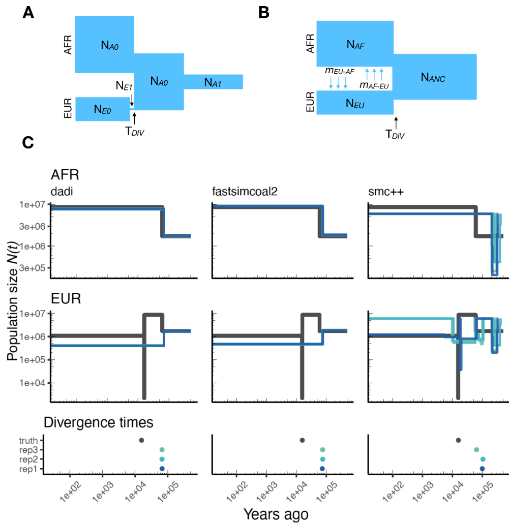
Appendix 1—figure 8. Parameters estimated using a two-population Drosophila model. Here, we show estimates of N(t) inferred using \hat{d}adi , fastsimcoal2 , and smc++ . Data were generated by simulating replicate Drosophila genomes under the Li and Stephan, 2006 model and using the genetic map inferred in Cameron et al., 2012 . See legend of Figure 4 for details. In shades of blue, we show the estimated N(t) trajectories for each replicate. In black we show the simulated population sizes.
